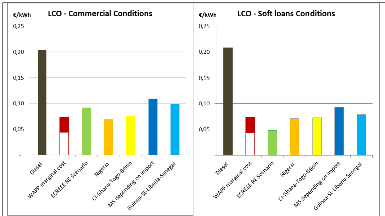
Figure 3: LCOE for various parts of the ECOWAS compared to diesel production and WAPP tariffs. (Commercial and soft loan condition)
